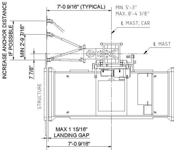
ELEVATION VIEW
